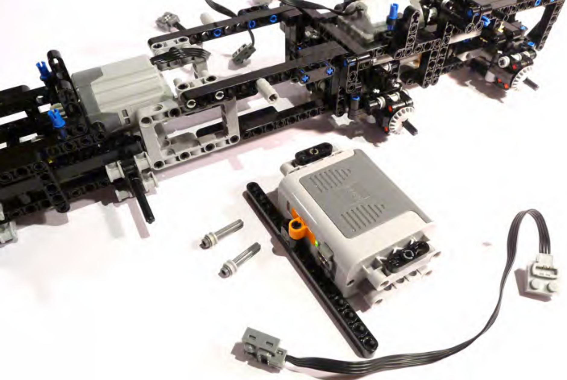
Extension wire connected between battery and IR reciever
